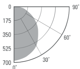
Indoor Distribution Curve
